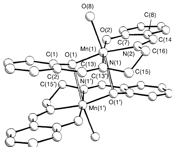
Fig. 1 Structure of the [\{\text{Mn}(\text{salen})(\text{H}_2\text{O})\}_2]^+ dimer; perchlorate anions, water of crystallisation and hydrogen atoms have been omitted for clarity. Selected interatomic distances (Å) and angles ( ^\circ ): Mn(1)–O(1) 1.891(3), Mn(1)–O(2) 1.866(3), Mn(1)–O(8) 2.208(3), Mn(1)–N(1) 1.975(4), Mn(1)–N(2) 1.972(4), Mn(1)–O(1') 2.490(3), Mn(1) \cdots Mn(1') 3.361(2), O(1)–Mn(1)–O(2) 94.2(1), O(1)–Mn(1)–O(8) 94.3(1), O(1)–Mn(1)–N(1) 90.5(1), O(1)–Mn(1)–N(2) 168.3(1), O(1)–Mn(1)–O(1') 80.7(1), where ' denotes -x, -y, -z .
